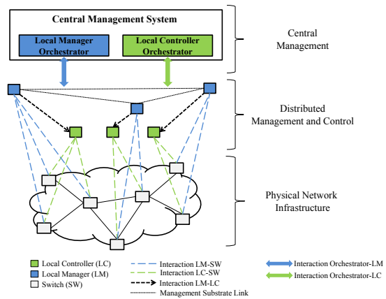
Fig. 1. Resource management and control framework proposed in [5].
